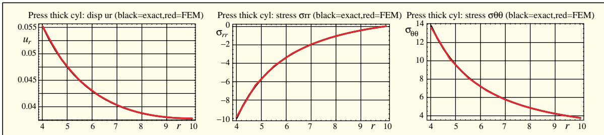
FIGURE 7.7. Pressurized thick cylinder benchmark: r plots of computed versus exact u_r , \sigma_{rr} and \sigma_{\theta\theta} for Quad8 meshes with \nu = 0 : (a) 2-element mesh, (b) 8-element mesh.
