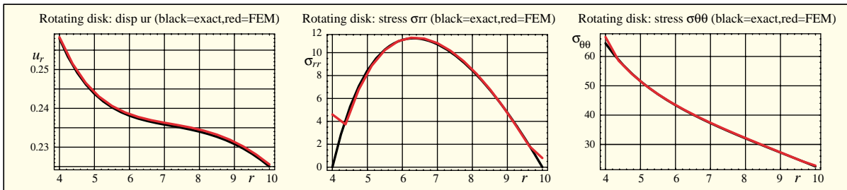
FIGURE 7.15. Rotating disk benchmark: radial plots of u_r , \sigma_{rr} and \sigma_{\theta\theta} for 4-element and 16-element Quad4, with Poisson ratio \nu = 1/3 .
