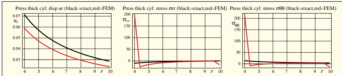
FIGURE 7.9. Pressurized thick cylinder benchmark: r plots of computed versus exact u_r , \sigma_{rr} and \sigma_{\theta\theta} for Quad4 meshes with \nu = 0.499 : (a) 4-element mesh, (b) 16-element mesh.
