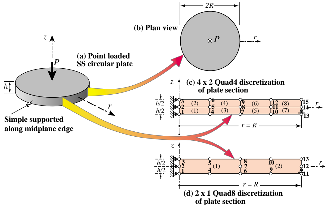
FIGURE 7.18. Point-loaded circular plate bending benchmark problem.
