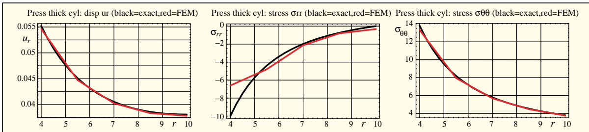
FIGURE 7.4. Pressurized thick cylinder benchmark: computed and exact nodal solution for 4-element Quad4 model with Poisson ratio \nu = 0 . The mesh is that shown in Figure 7.2(b).
