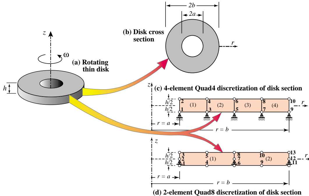
FIGURE 7.12. Rotating thin disk benchmark problem.
