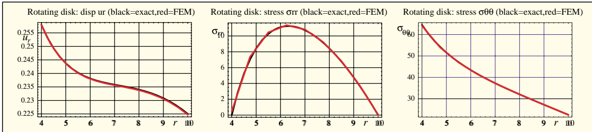
FIGURE 7.17. Rotating disk benchmark: radial plots of u_r , \sigma_{rr} and \sigma_{\theta\theta} for 2-element and 8-element Quad8 meshes, with Poisson ratio \nu = 1/3 .
