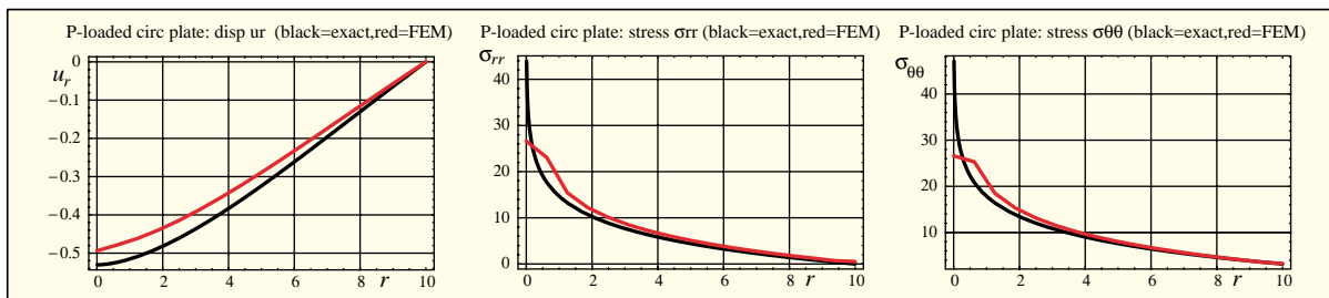
FIGURE 7.21. Point loaded circular plate benchmark: radial plots of u_r , \sigma_{rr} and \sigma_{\theta\theta} for 4 \times 2 and 16 \times 2 element Quad4, with Poisson ratio \nu = 1/3 . Plot is along the bottom plate surface z = -h/2 .
