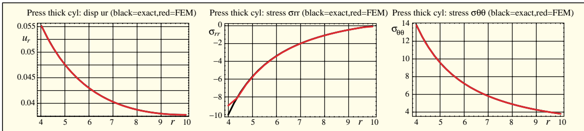
FIGURE 7.5. Pressurized thick cylinder benchmark: r plots of computed versus exact u_r , \sigma_{rr} and \sigma_{\theta\theta} for Quad4 meshes with \nu = 0 : (a) 4-element mesh, (b) 16-element mesh.
