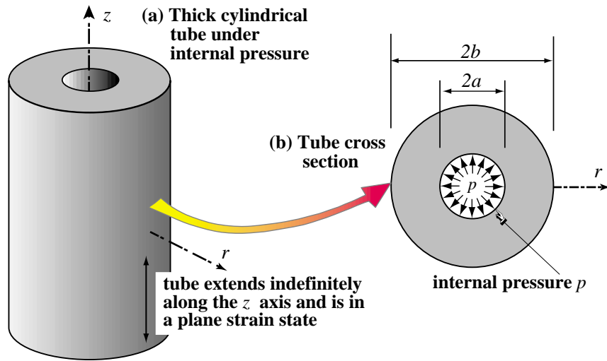
FIGURE 7.1. Pressurized thick cylinder benchmark problem. Reproduced from Figure 6.1 for convenience.
