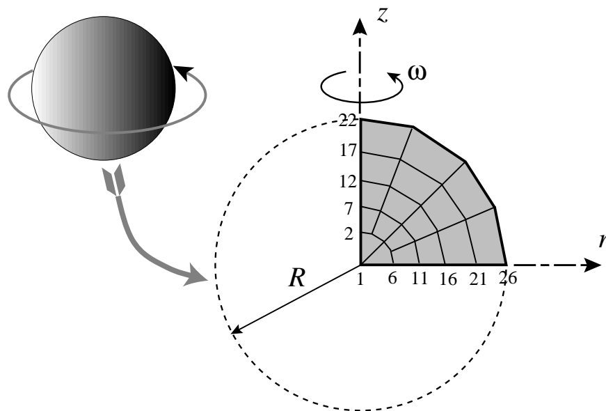
Figure E7.2. Our spinning planet.
