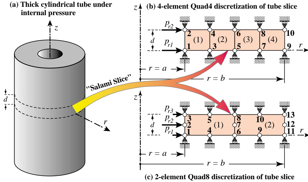
FIGURE 7.2. Two example FEM discretizations for the pressurized thick cylinder benchmark.
